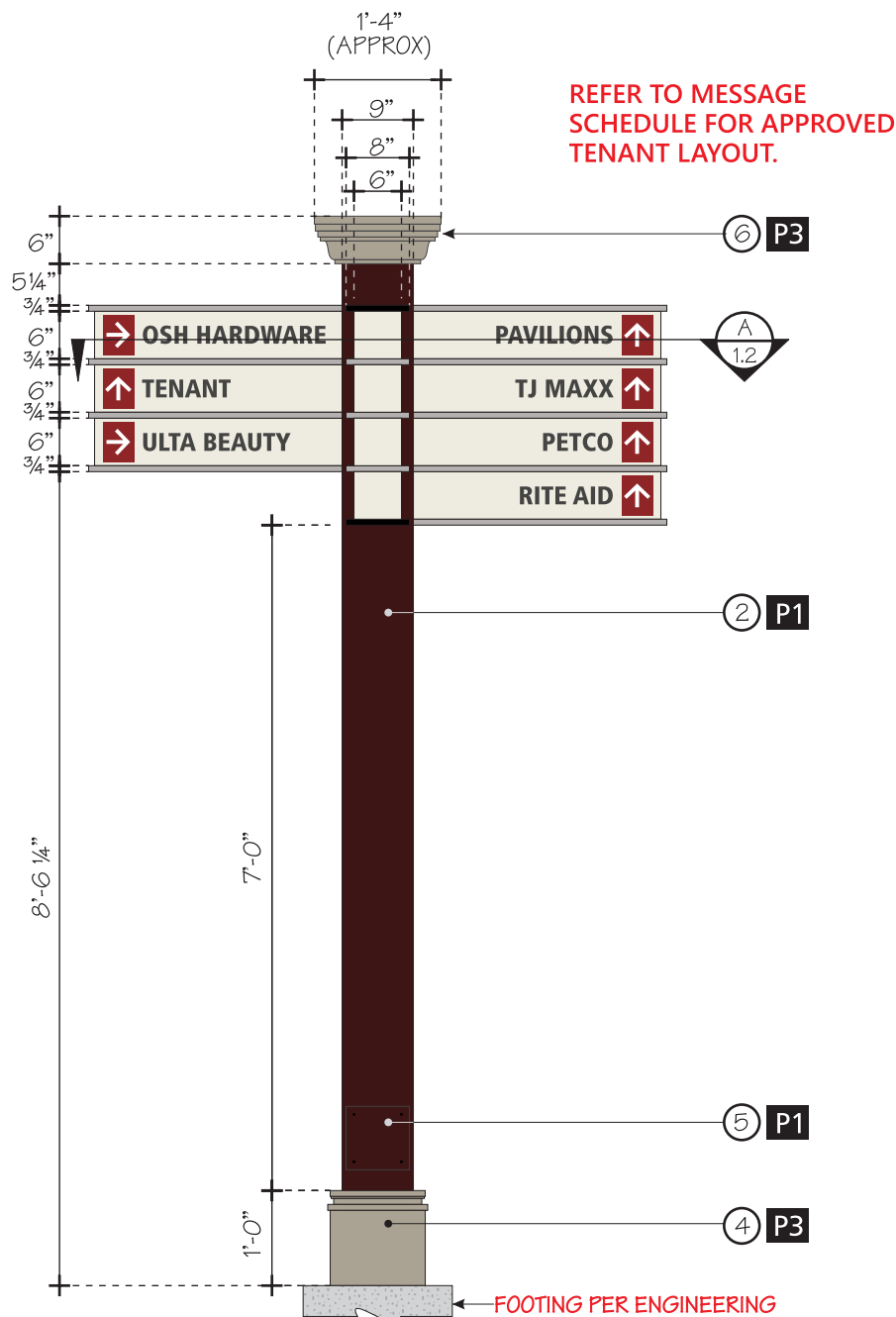
2 FRONT VIEW SCALE: 1/2" = 1'-0"
