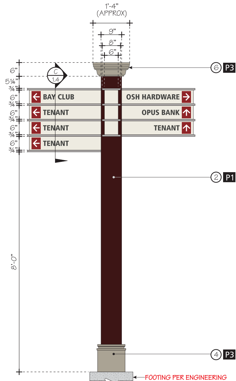
3 BACK SIDE VIEW SCALE: 1/2" = 1'-0"
