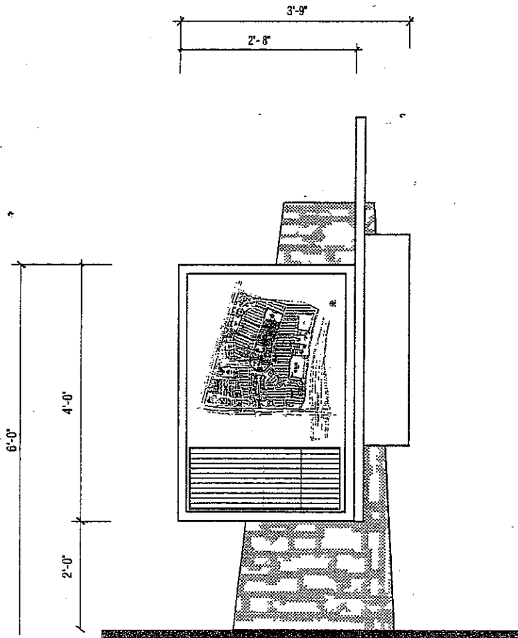
E NEIGHBORHOOD DISTRICT DIRECTORY (TYPICAL)
