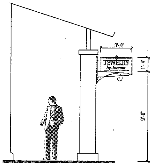
(F) NEIGHBORHOOD DISTRICT UNDER CANOPY - TENANT ID BLADE SIGN
