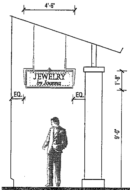
NEIGHBORHOOD DISTRICT UNDER CANOPY - TENANT HANGING SIGN
