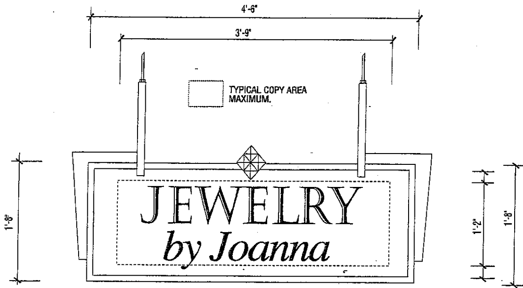
DOUBLE FACED - NON-ILLUMINATED
