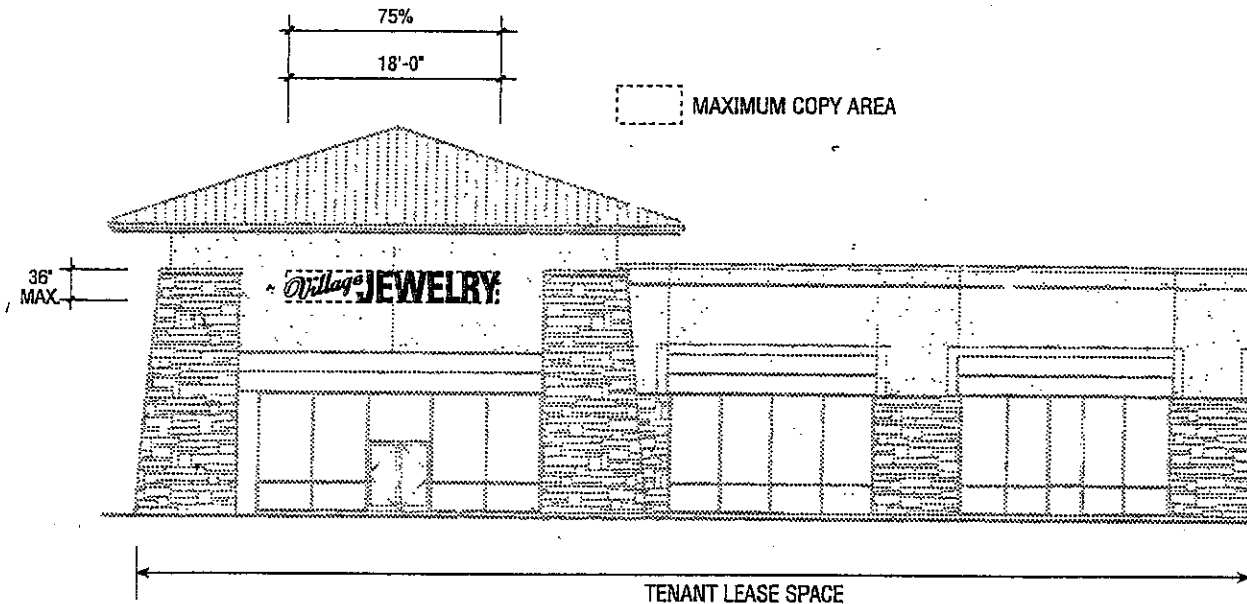
D NEIGHBORHOOD DISTRICT PAD TENANT I.D. WALL SIGNS (TYPICAL)
